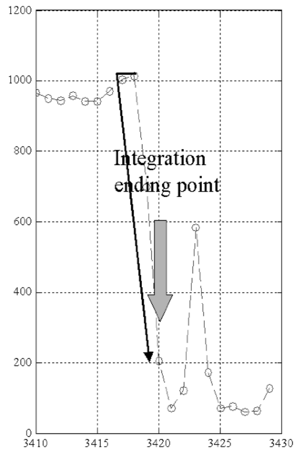
Figure 3.3.5. Sample tension vs. time data showing the rupture point at which integration of energy ends.
